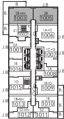
KEYPLAN 10TH
