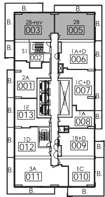
KEYPLAN 38-40TH
